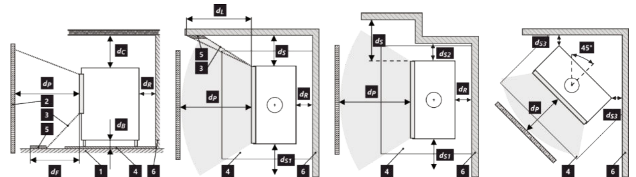
Fig. 2 Safe distances from flammable materials
