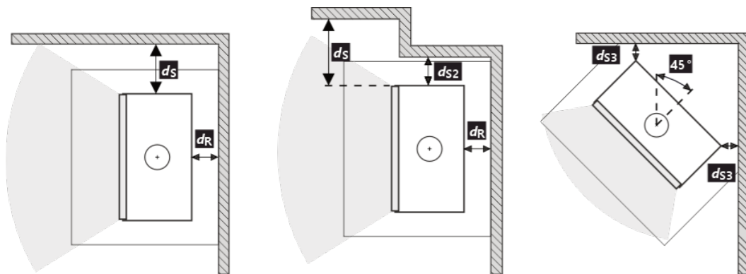
Fig. 3 Safe distances from nonflammable materials
