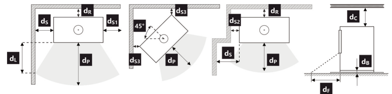
Fig. 2 Safe distances from flammable materials
