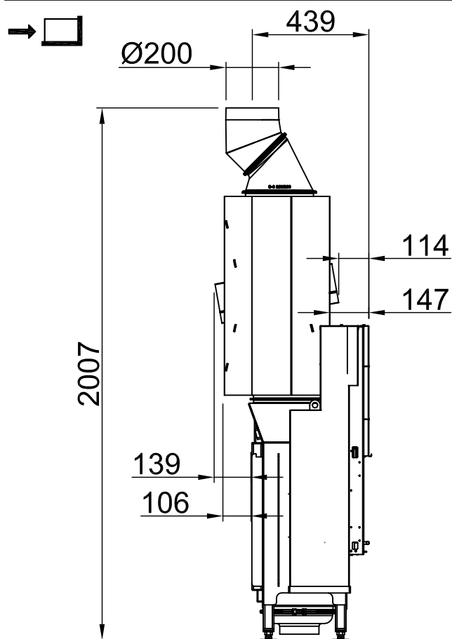
~1:20 Thermobox, schmal
